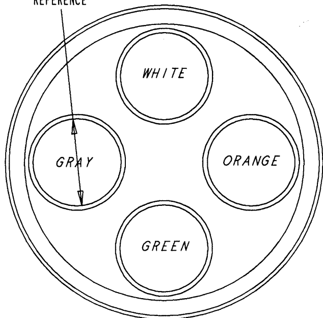
SPIGOT END VIEW
